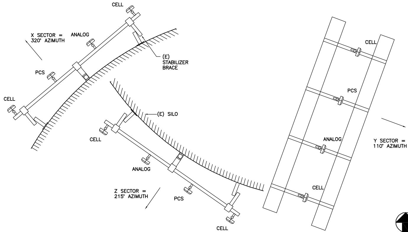
2 EXISTING ANTENNA CONFIGURATION
