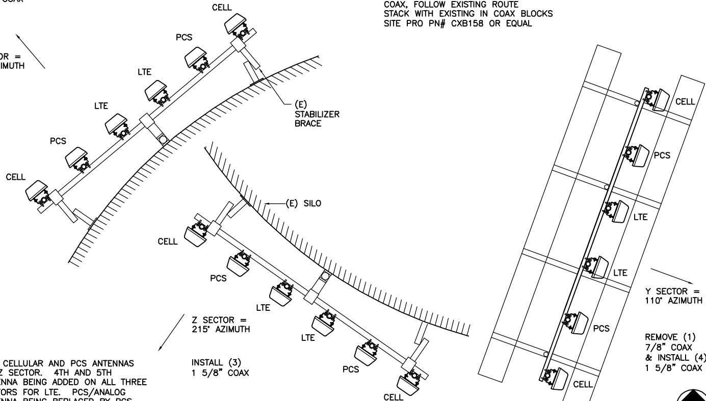
1 PROPOSED ANTENNA CONFIGURATION
